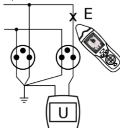
Fig. 8 Diagram of the voltage mode.
